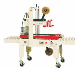
AS523 Carton Sealing Machine 半自动封箱机 Power Supply/供给电源: 110V/220-240V/50-60Hz Power/功率: 240W Conveyor Speed/输送速度: 20m/min Max. Carton Size/最大纸箱尺寸: W500xH500mm Min. Carton Size/最小纸箱尺寸: W100xH80mm Width Of Tape/胶带宽度: 50mm or 60mm Option: 3inch tape & overlap (Model AS523/3)
